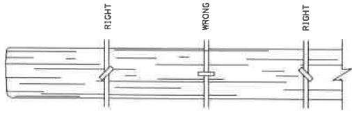
DO NOT DRIVE STAPLES PARALLEL TO SIDE OF POST
