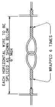
SPLICE DETAIL FOR BARBED WIRE/WIRE MESH FENCE
